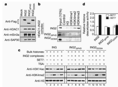
Figure 2. Methylated H3K4 recognition by the ING2 PHD domain enhances ING2-associated HDAC1 histone deacetylase activity in vitro
